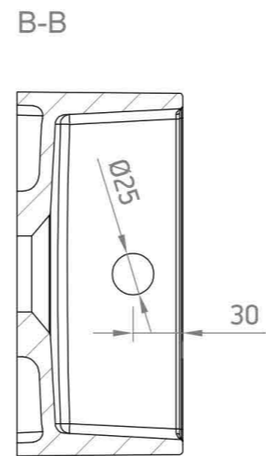
Backside view
